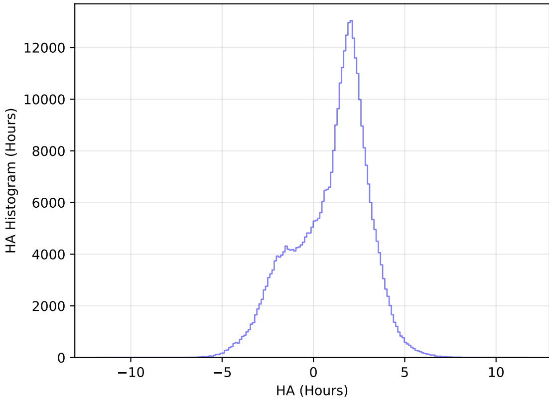
internal_u_expt38_nscale0.9v3.4_10yrs All sky y band: HA Histogram
