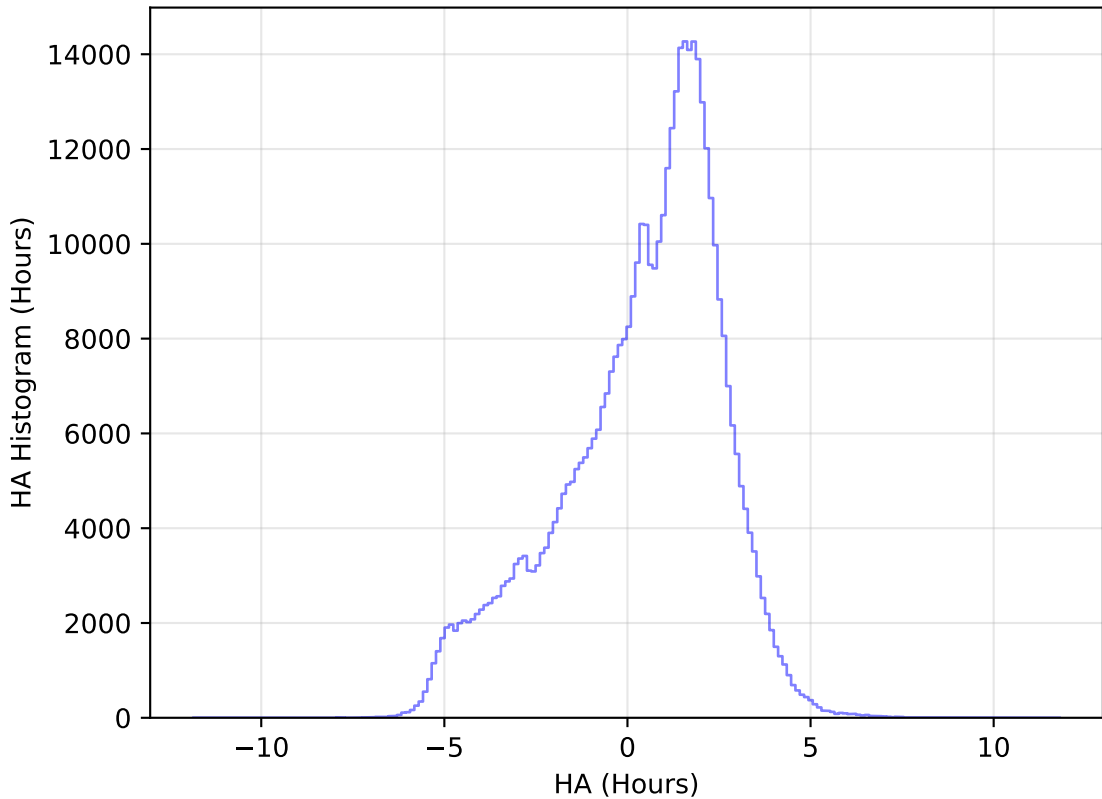
internal_u_expt38_nscale0.9v3.4_10yrs All sky r band: HA Histogram
