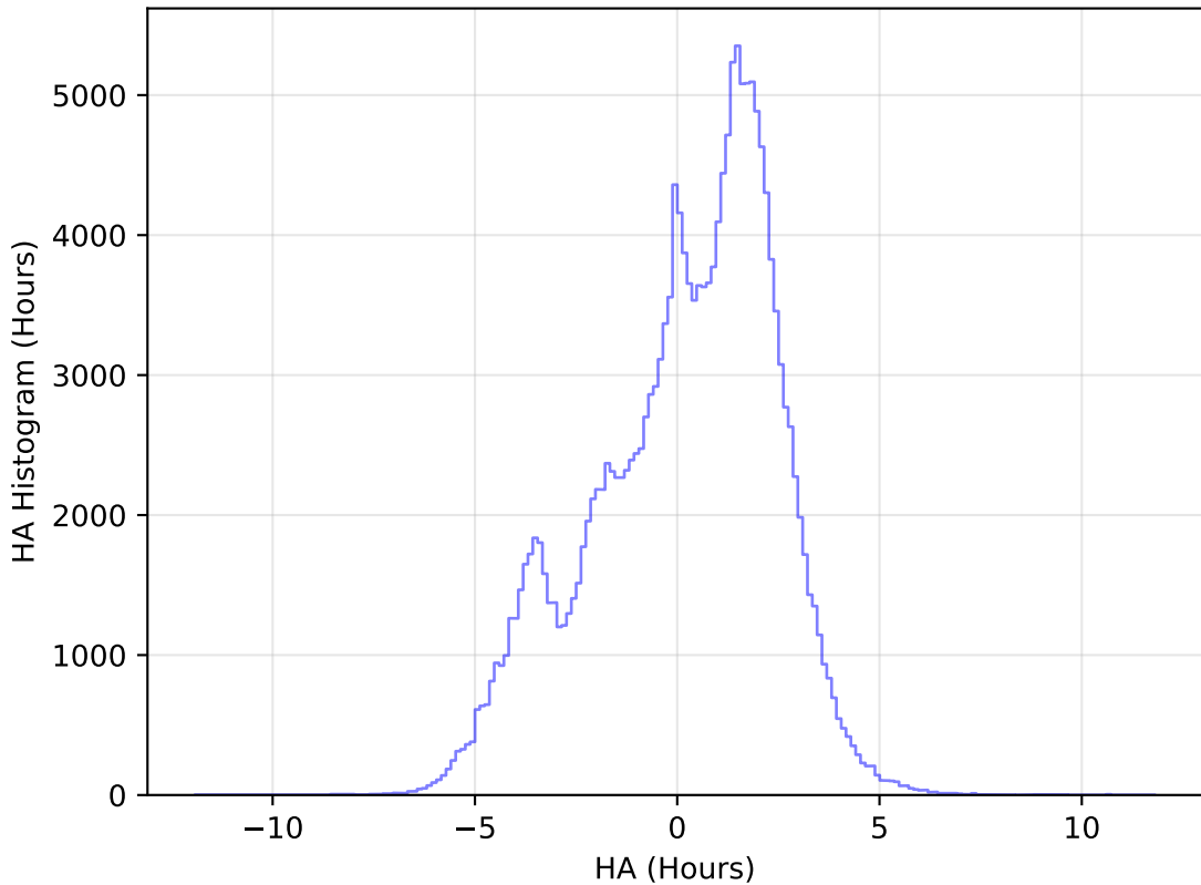
internal_u_expt38_nscale0.9v3.4_10yrs All sky g band: HA Histogram
