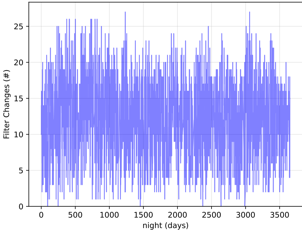
internal_u_expt38_nscale0.9v3.4_10yrs Per Night: Filter Changes
