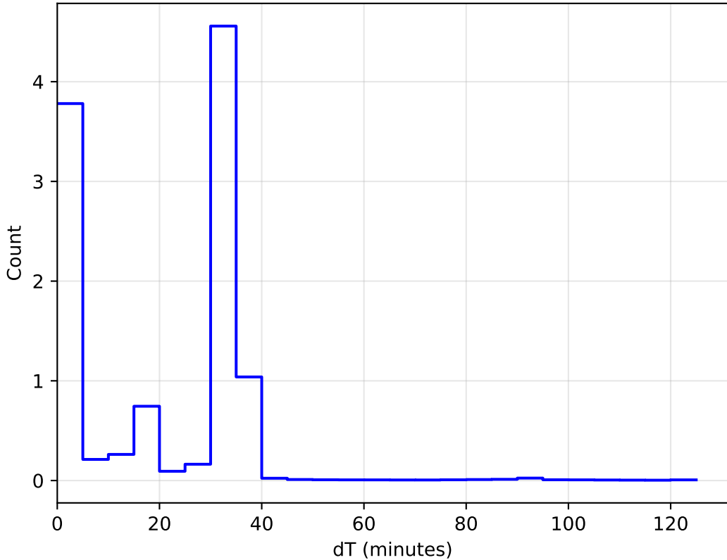
internal_u_expt38_nscale0.9v3.4_10yrs WFD: DeltaT Histogram
