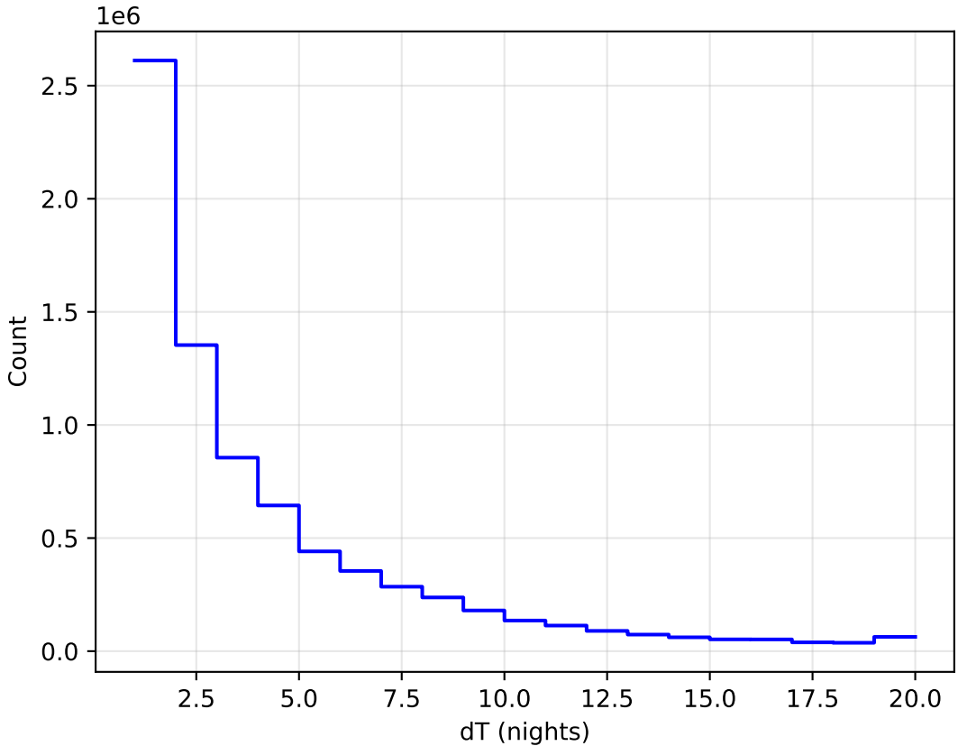
internal_u_expt38_nscale0.9v3.4_10yrs WFD all bands: DeltaNight Histogram
