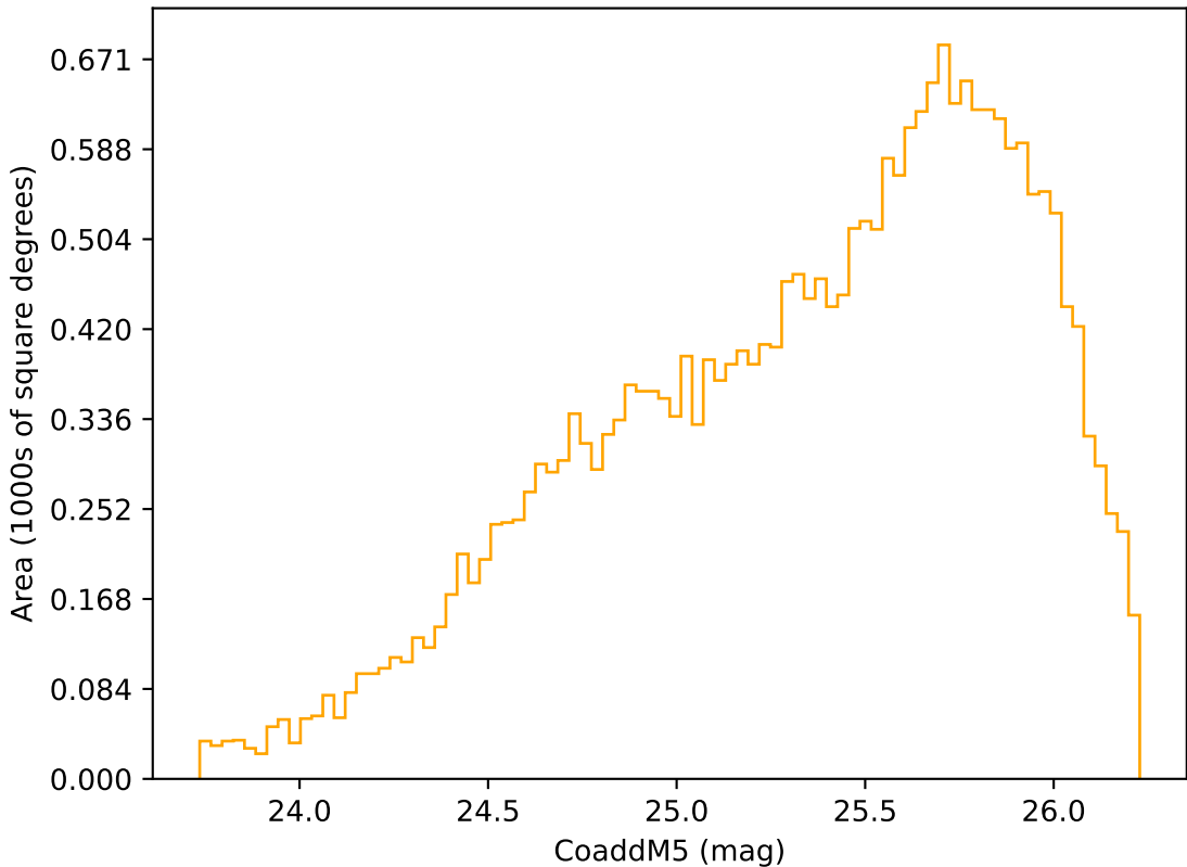
internal_u_expt38_nscale0.9v3.4_10yrs Yr 3-4 r band: CoaddM5
