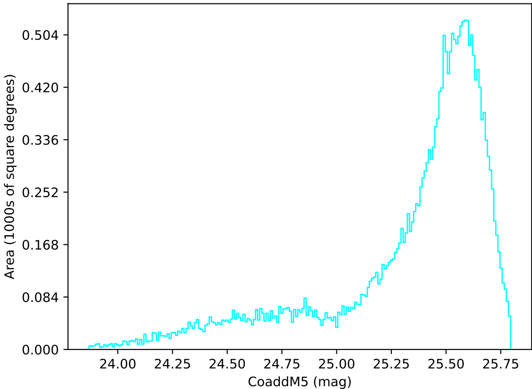
internal_u_expt38_nscale0.9v3.4_10yrs All sky u band: CoaddM5
