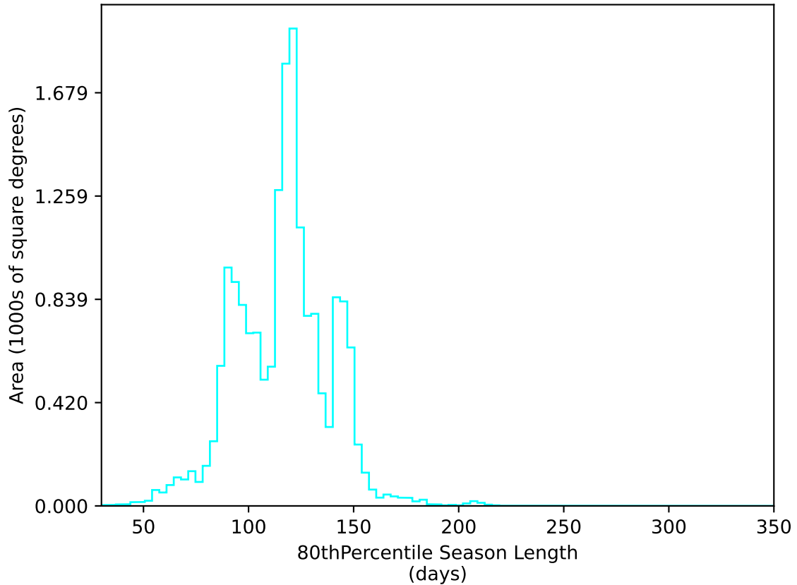
internal_u_expt38_nscale0.9v3.4_10yrs WFD u band: 80thPercentile Season Length
