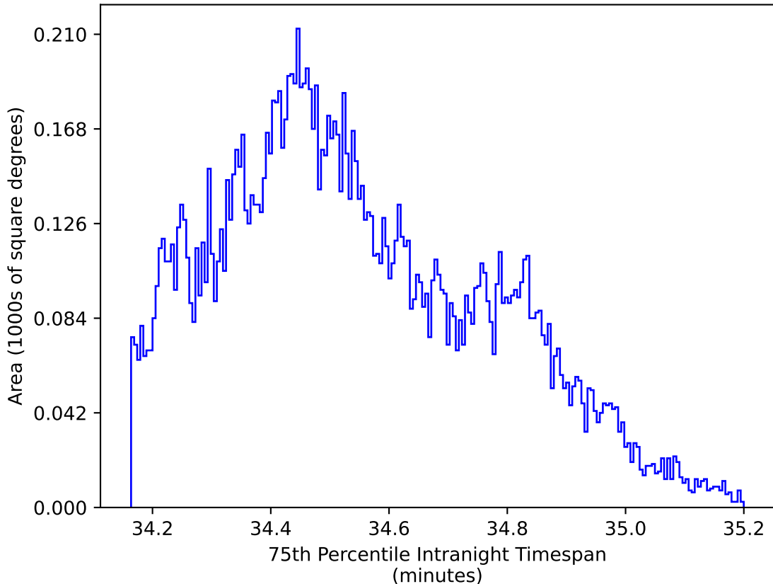
internal_u_expt38_nscale0.9v3.4_10yrs WFD zy bands: 75th Percentile Intranight Timespan
