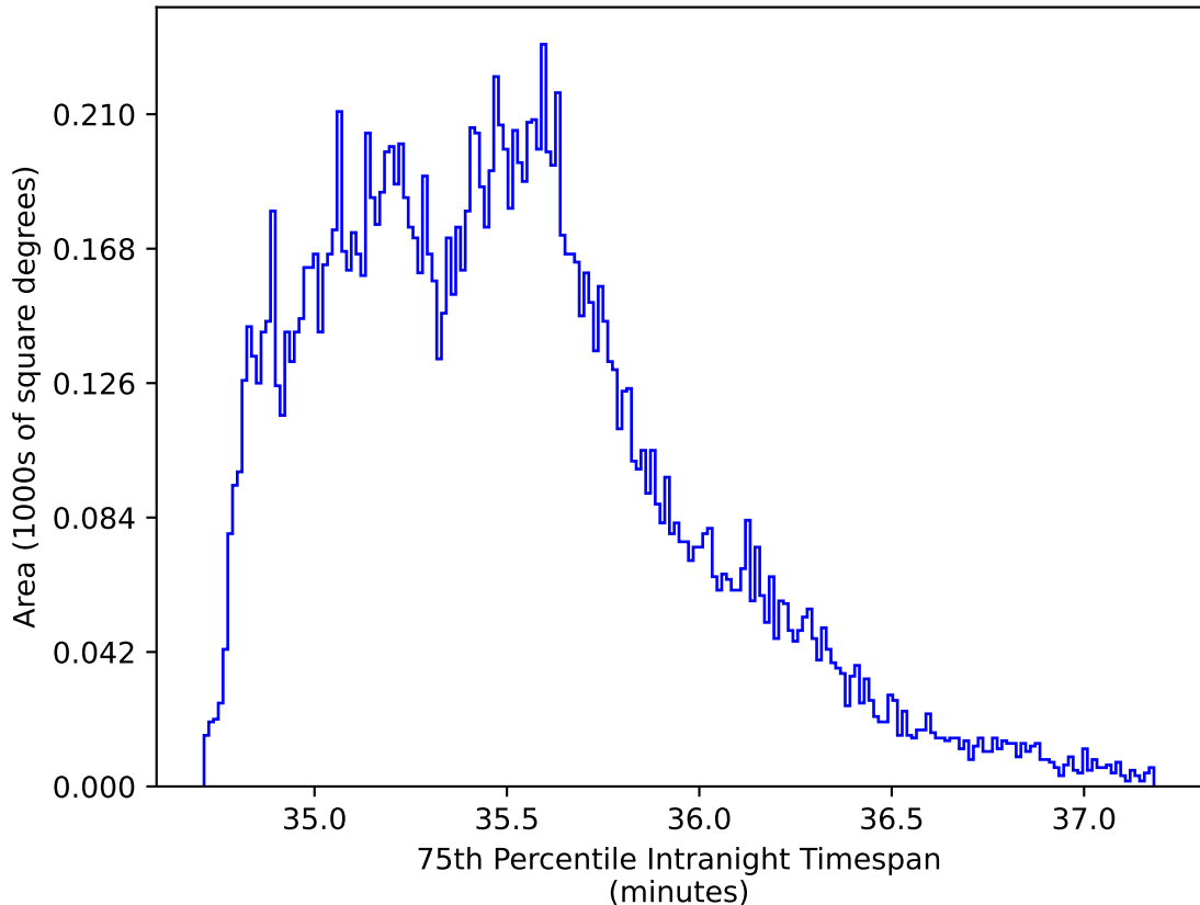
internal_u_expt38_nscale0.9v3.4_10yrs WFD all bands: 75th Percentile Intranight Timespan
