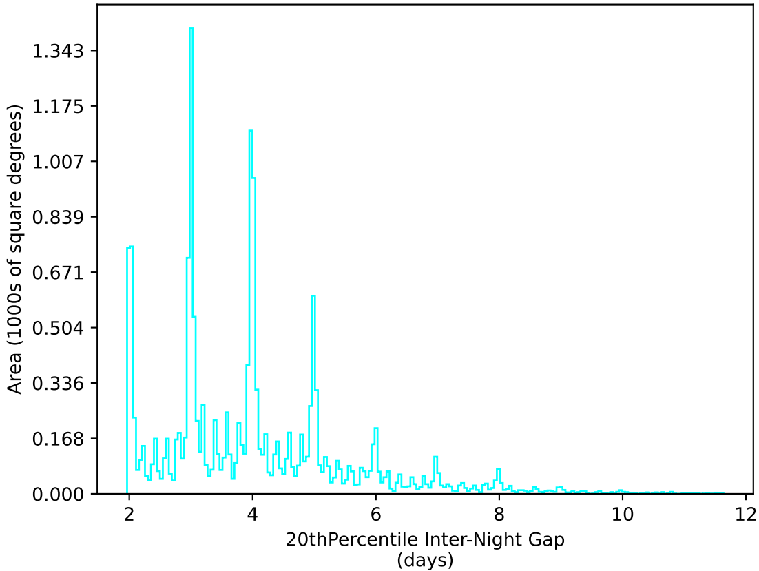
internal_u_expt38_nscale0.9v3.4_10yrs WFD u band: 20thPercentile Inter-Night Gap
