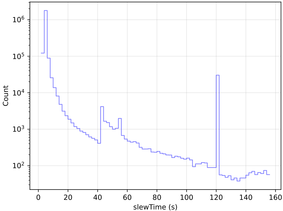
internal_u_expt38_nscale0.9v3.4_10yrs All visits: Slew Time Histogram
