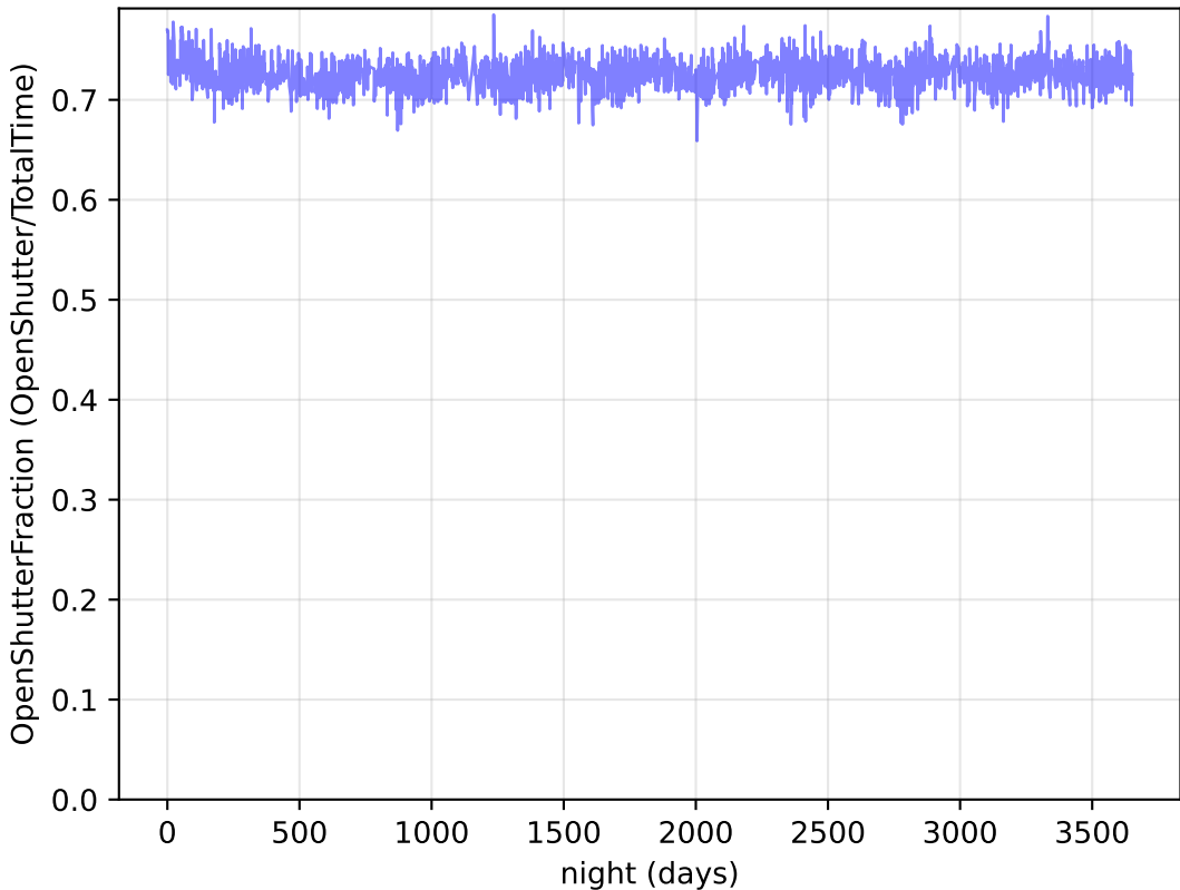
internal_u_expt38_nscale0.9v3.4_10yrs : OpenShutterFraction
