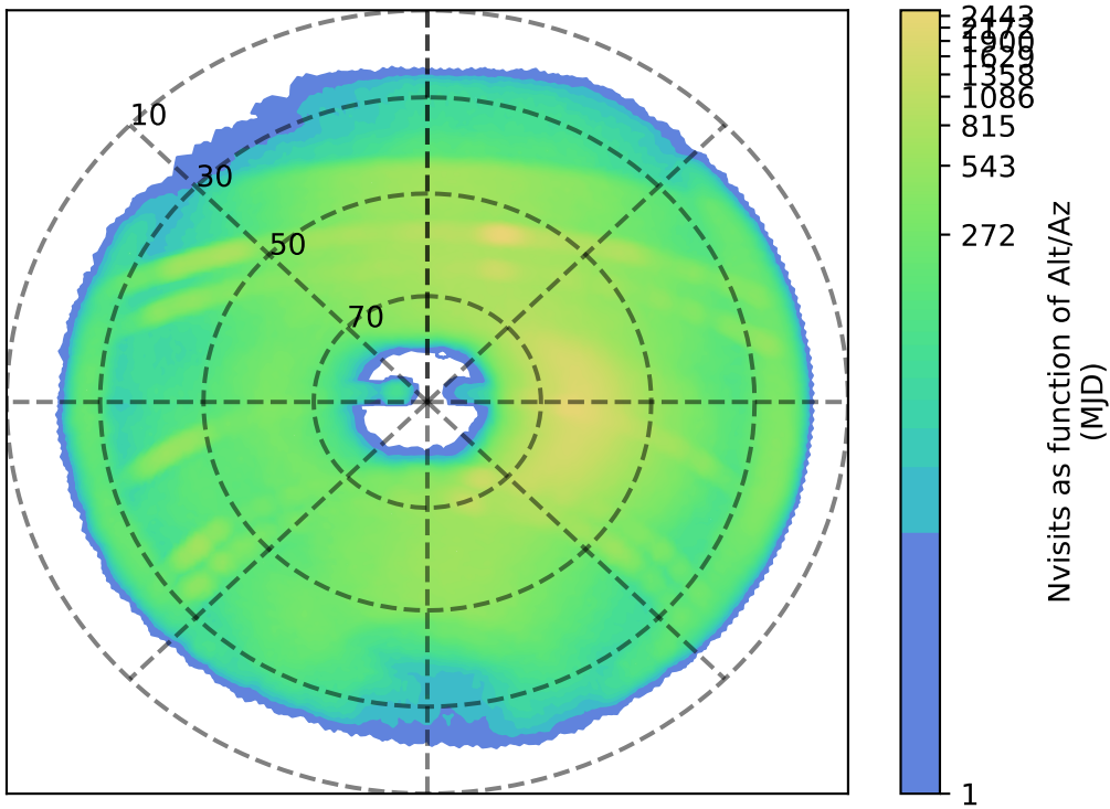
internal_u_expt38_nscale0.9v3.4_10yrs z: Nvisits as function of Alt/Az
