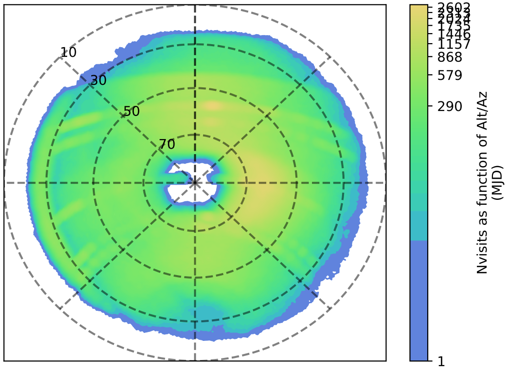
internal_u_expt38_nscale0.9v3.4_10yrs r: Nvisits as function of Alt/Az
