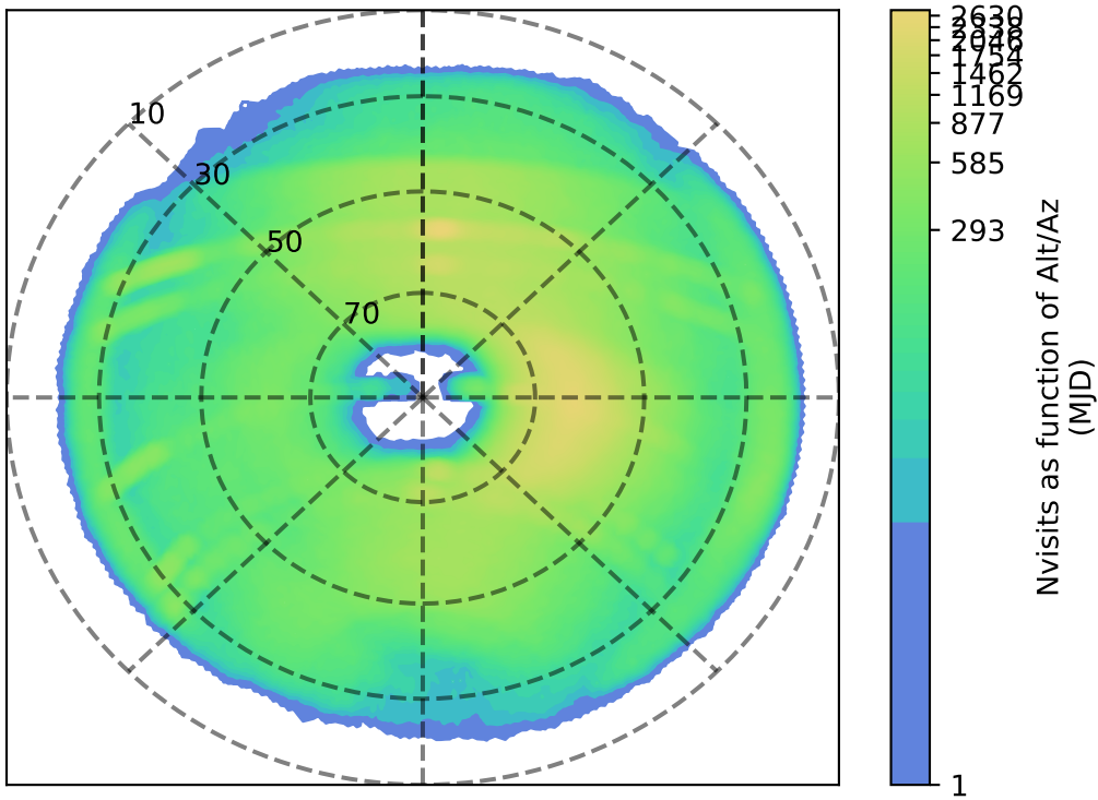
internal_u_expt38_nscale0.9v3.4_10yrs i: Nvisits as function of Alt/Az
