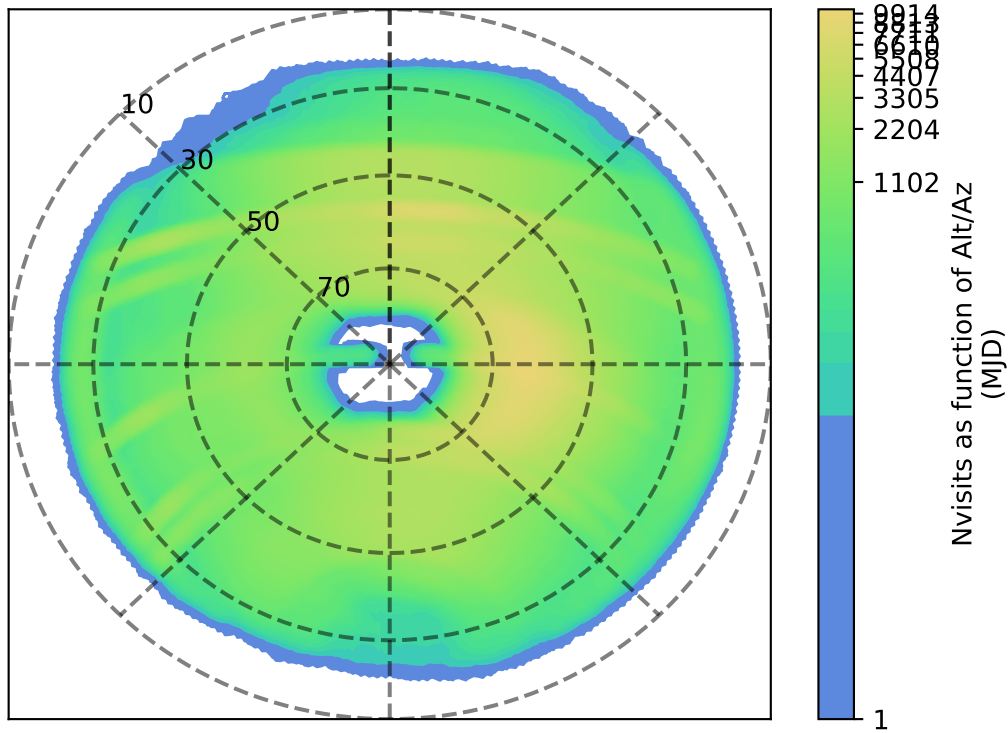
internal_u_expt38_nscale0.9v3.4_10yrs : Nvisits as function of Alt/Az
