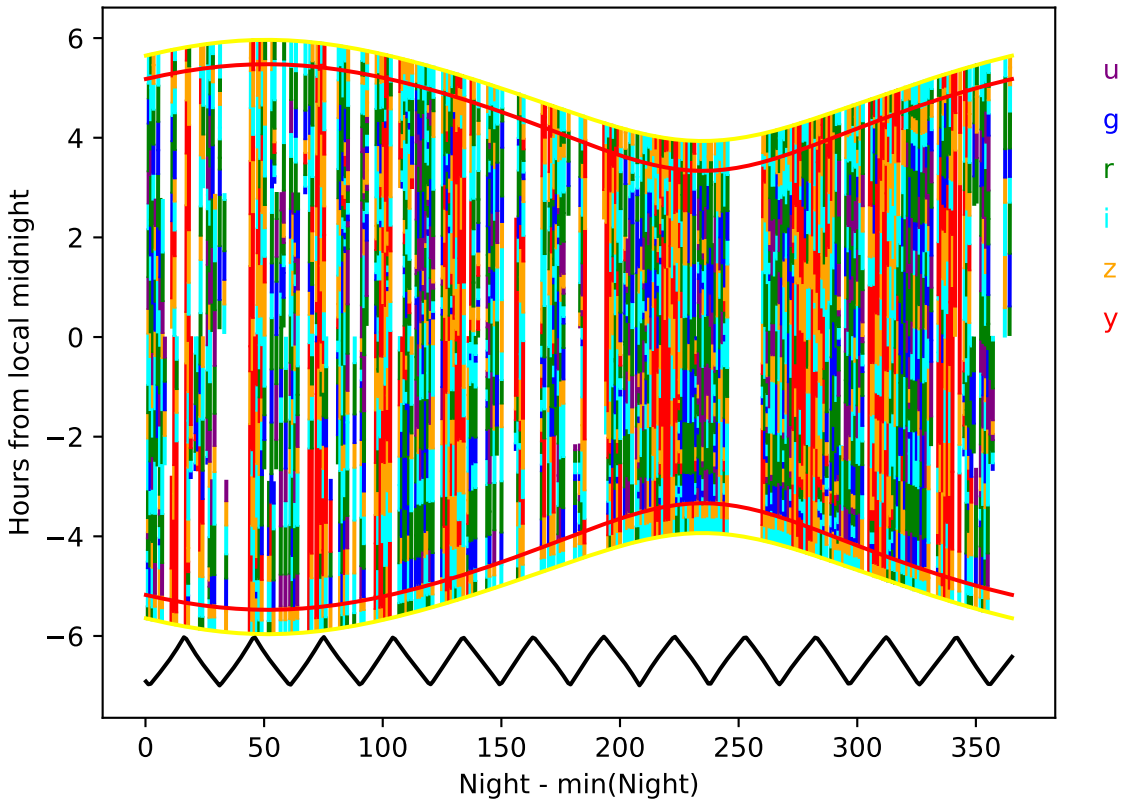
internal_u_expt38_nscale0.9v3.4_10yrs year 5-6: Hourglass
