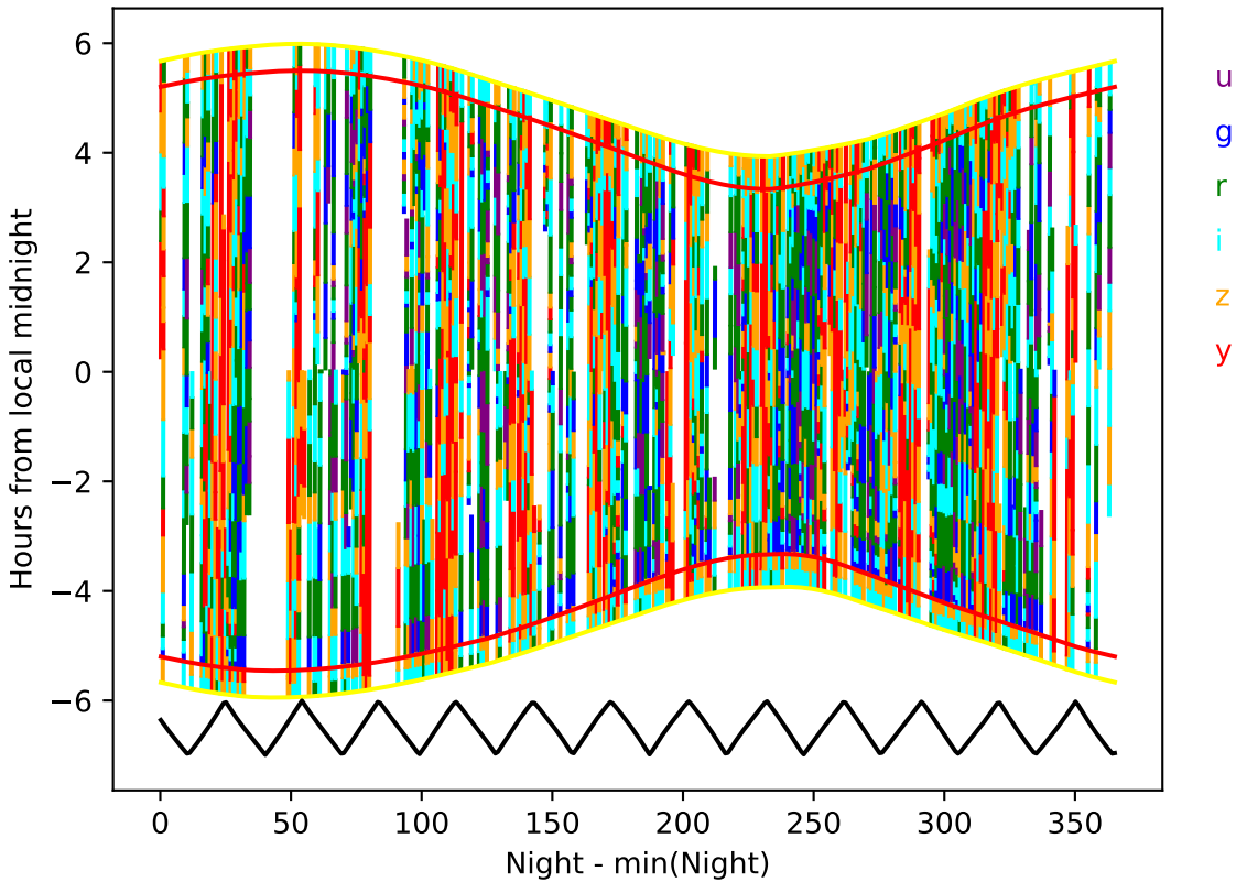
internal_u_expt38_nscale0.9v3.4_10yrs year 4-5: Hourglass
