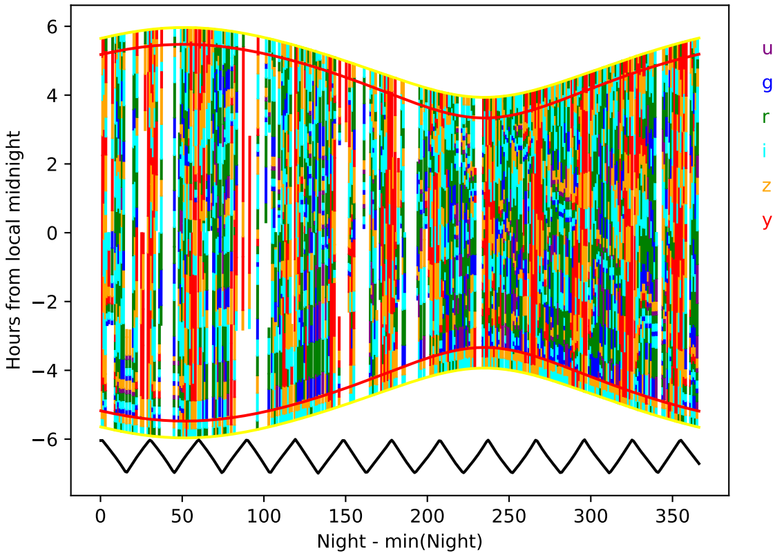
internal_u_expt38_nscale0.9v3.4_10yrs year 1-2: Hourglass
