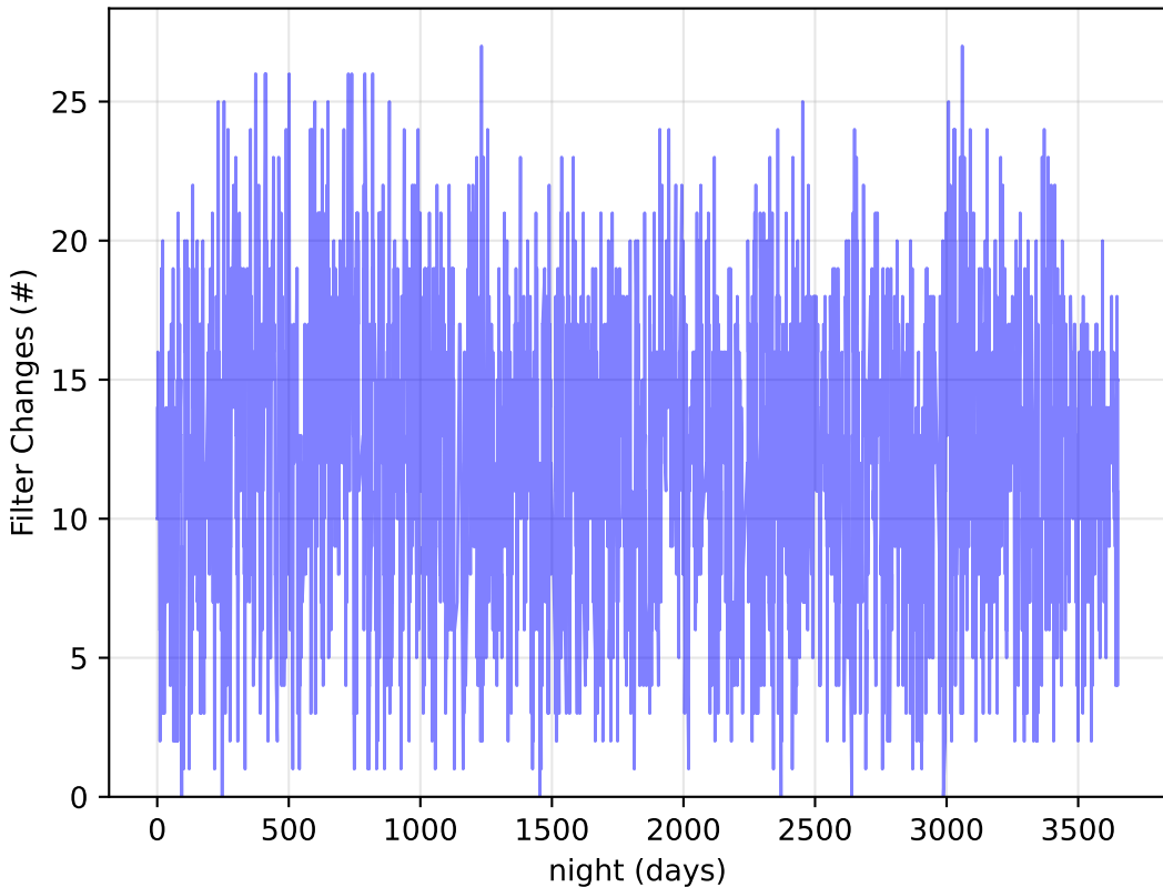
internal_u_expt38_nscale0.9v3.4_10yrs : Filter Changes
