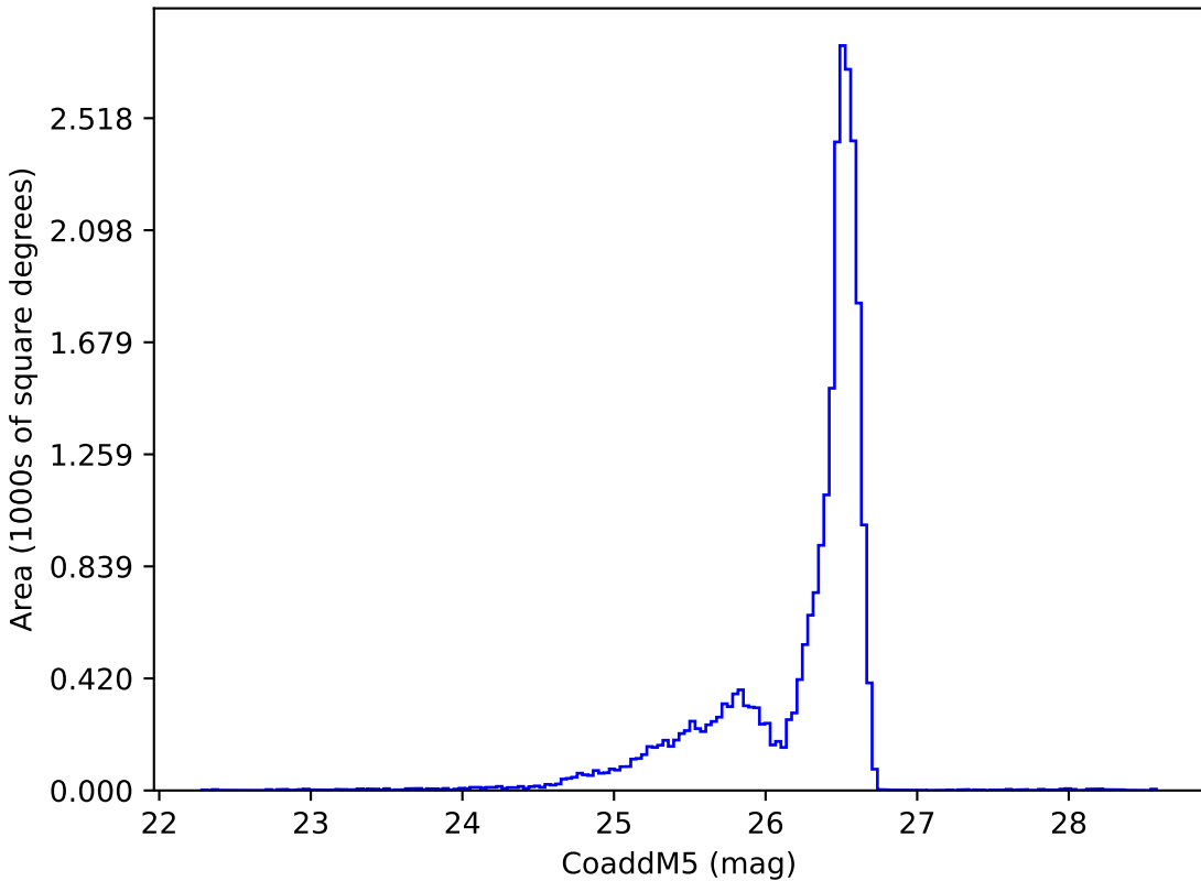
internal_u_expt38_nscale0.9v3.4_10yrs i: CoaddM5
