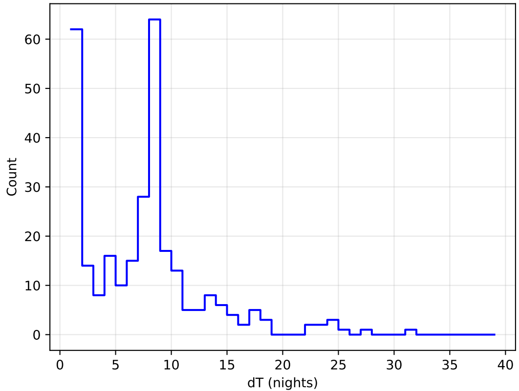
internal_u_expt38_nscale0.9v3.4_10yrs all bands: DD:XMM_LSS Delta Nights Histogram
