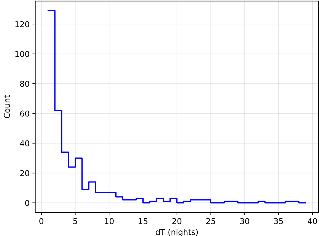
internal_u_expt38_nscale0.9v3.4_10yrs all bands: DD:WFD Delta Nights Histogram
