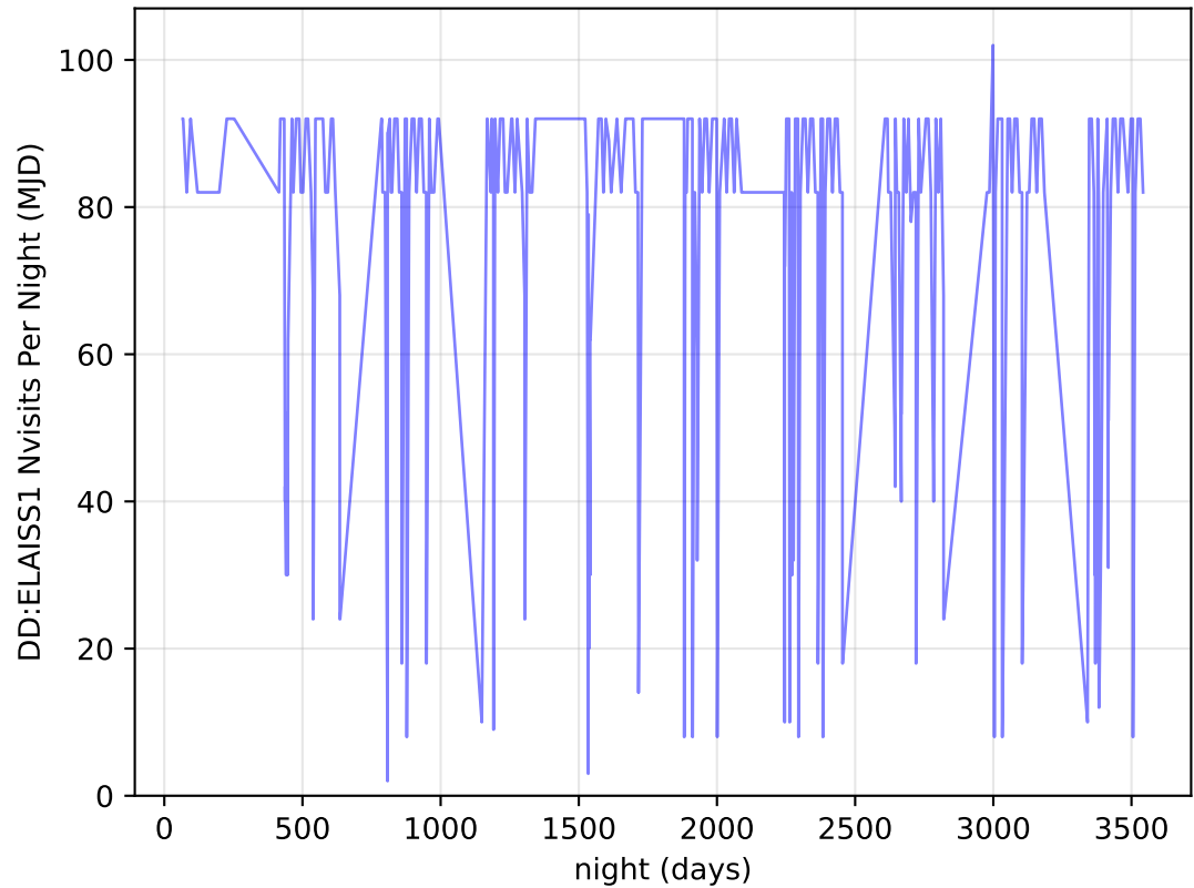
internal_u_expt38_nscale0.9v3.4_10yrs all bands: DD:ELAISS1 Nvisits Per Night
