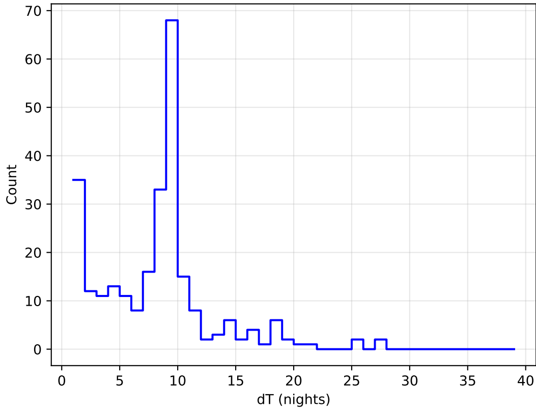
internal_u_expt38_nscale0.9v3.4_10yrs all bands: DD:ELAISS1 Delta Nights Histogram
