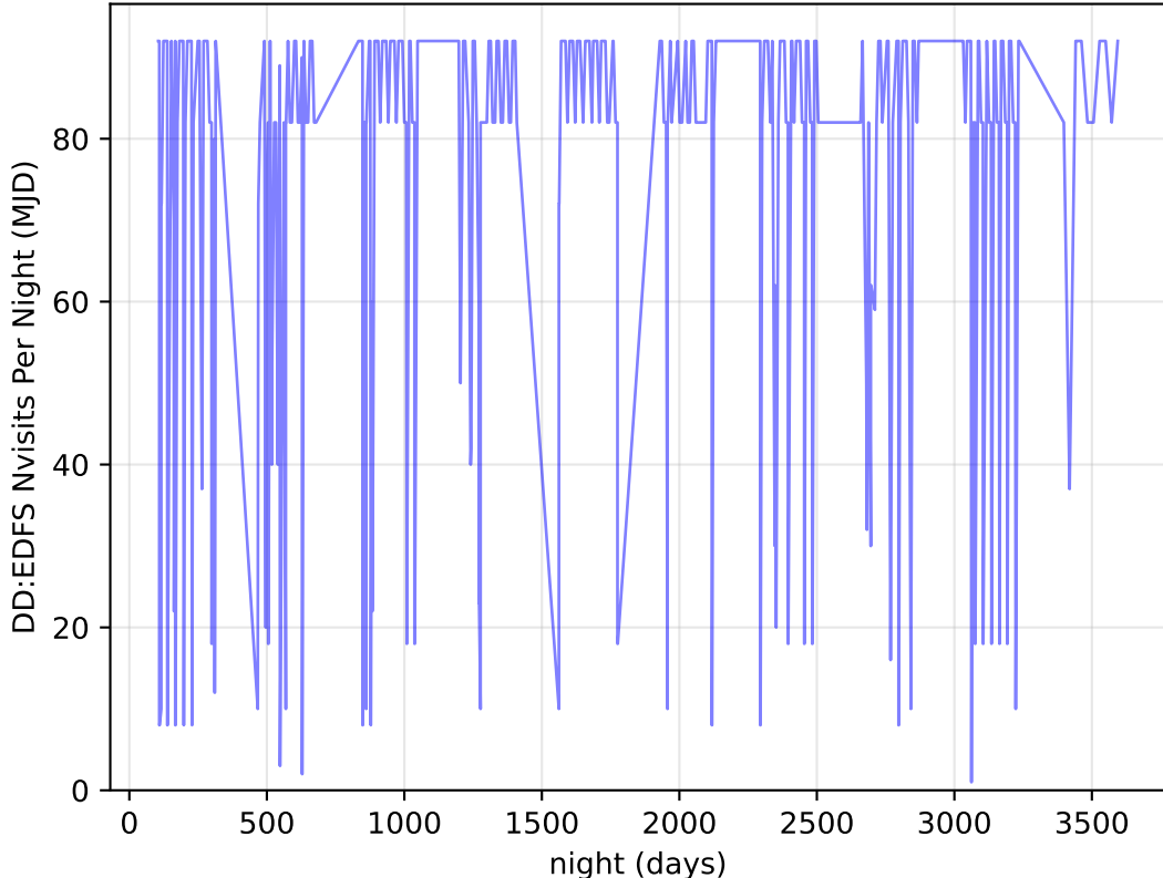
internal_u_expt38_nscale0.9v3.4_10yrs all bands: DD:EDFS Nvisits Per Night
