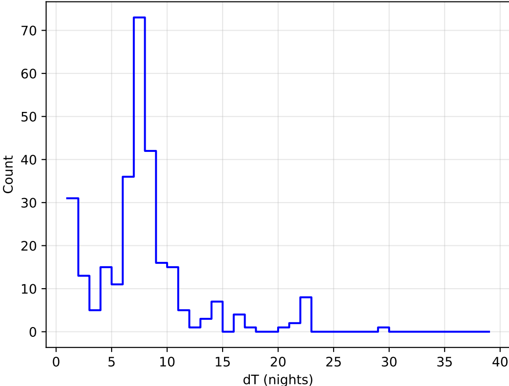
internal_u_expt38_nscale0.9v3.4_10yrs all bands: DD:EDFS Delta Nights Histogram
