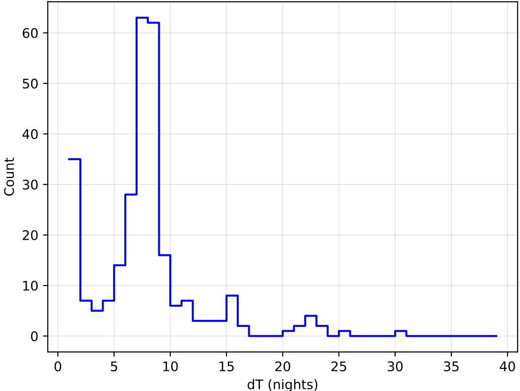
internal_u_expt38_nscale0.9v3.4_10yrs all bands: DD:ECDFS Delta Nights Histogram
