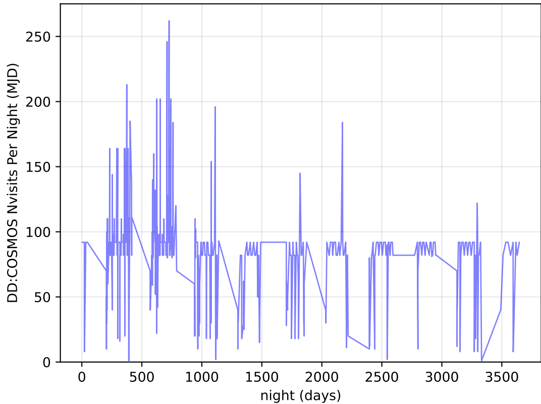
internal_u_expt38_nscale0.9v3.4_10yrs all bands: DD: COSMOS Nvisits Per Night
