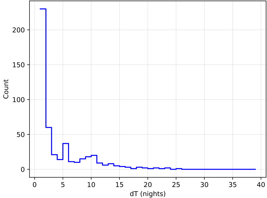
internal_u_expt38_nscale0.9v3.4_10yrs all bands: DD:COSMOS Delta Nights Histogram
