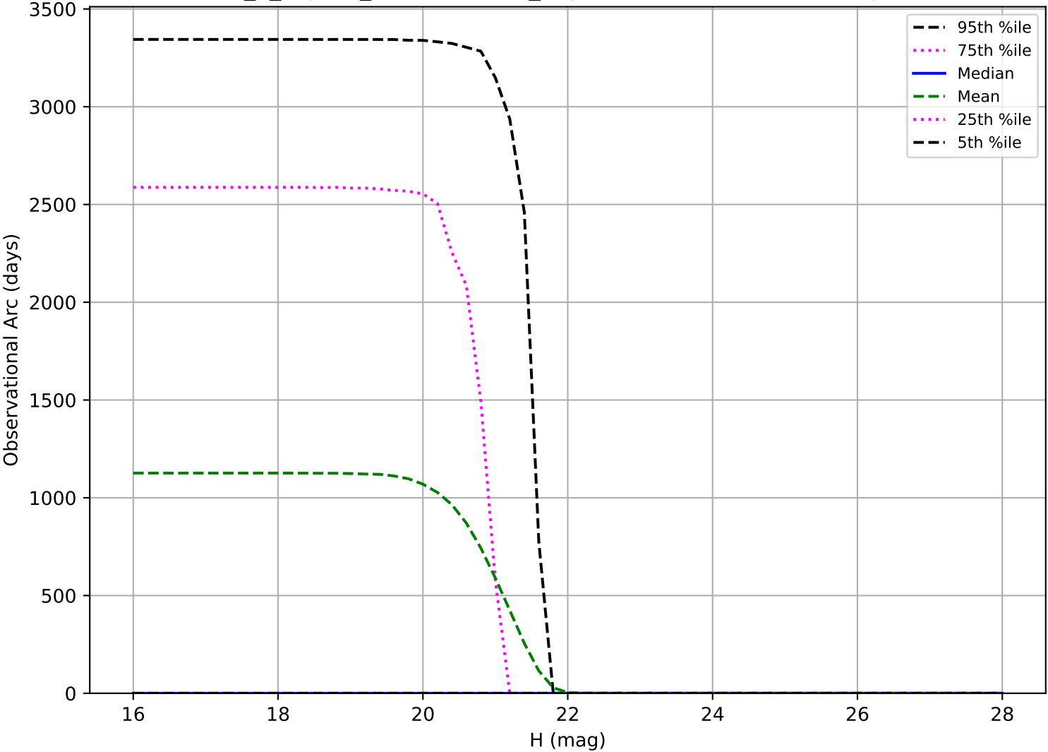
internal_u_expt30_nscale1.5v3.4_10yrs: Observational Arc Length Vatra
