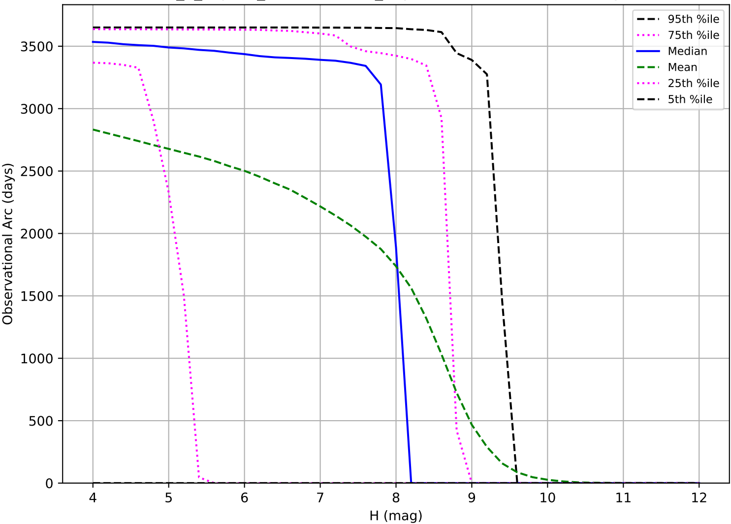
internal_u_expt30_nscale1.5v3.4_10yrs: Observational Arc Length TNO
