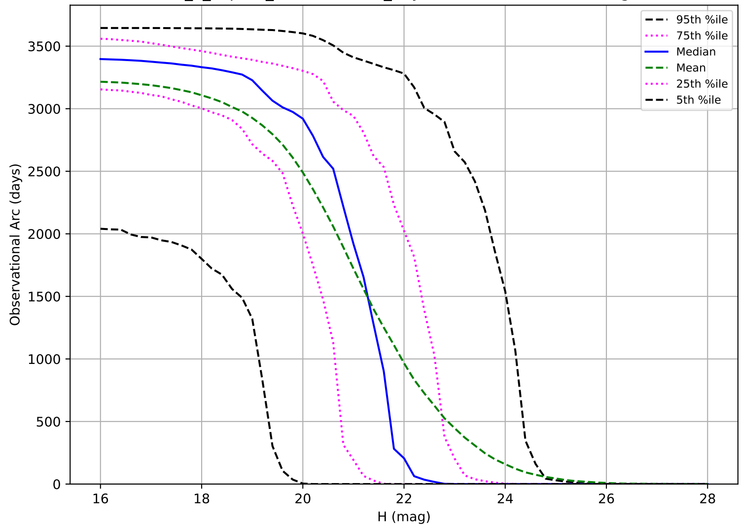
internal_u_expt30_nscale1.5v3.4_10yrs: Observational Arc Length PHA
