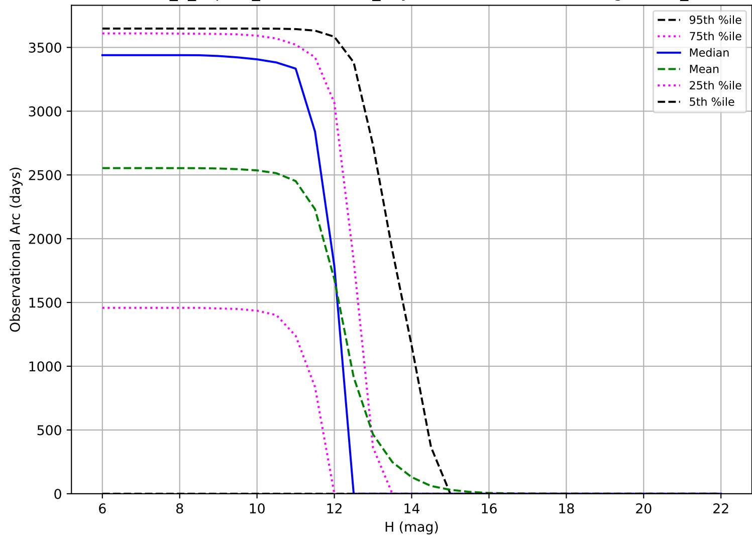
internal_u_expt30_nscale1.5v3.4_10yrs: Observational Arc Length OCC_r20
