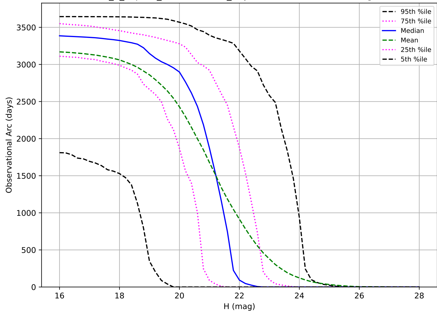
internal_u_expt30_nscale1.5v3.4_10yrs: Observational Arc Length NEO
