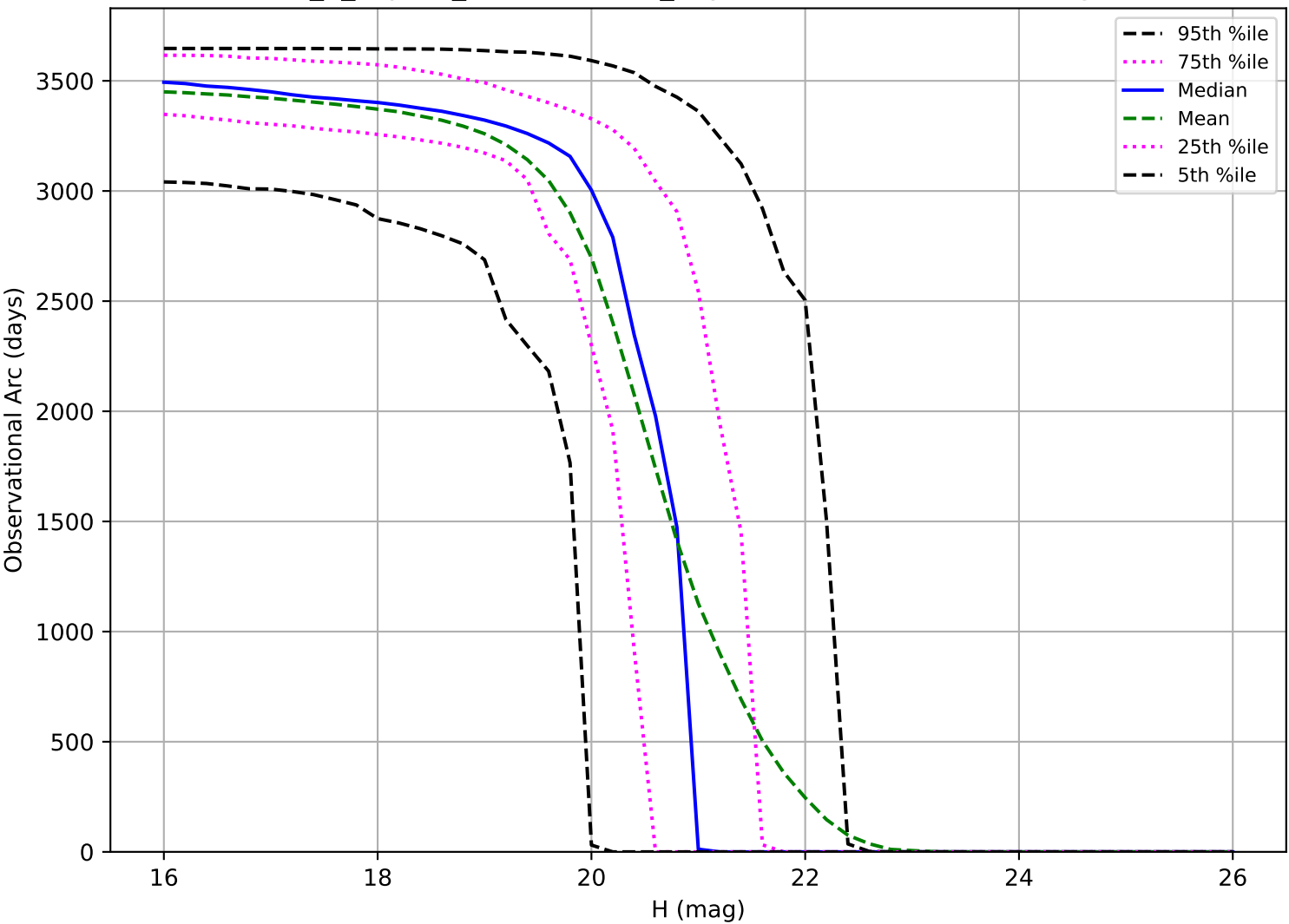
internal_u_expt30_nscale1.5v3.4_10yrs: Observational Arc Length MBA
