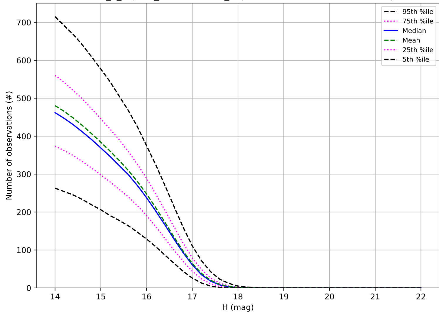
internal_u_expt30_nscale1.5v3.4_10yrs: Number of observations Trojan
