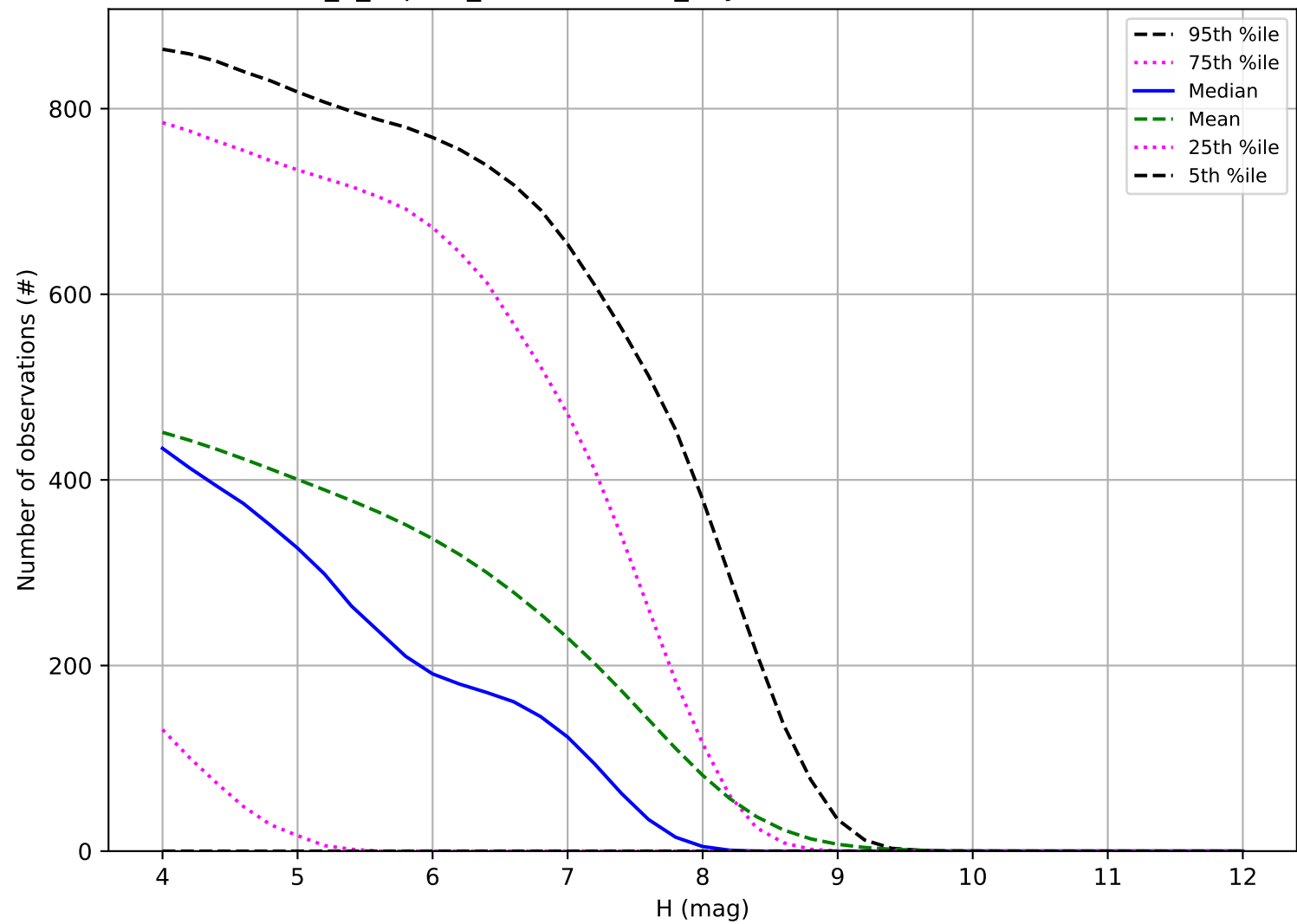
internal_u_expt30_nscale1.5v3.4_10yrs: Number of observations TNO
