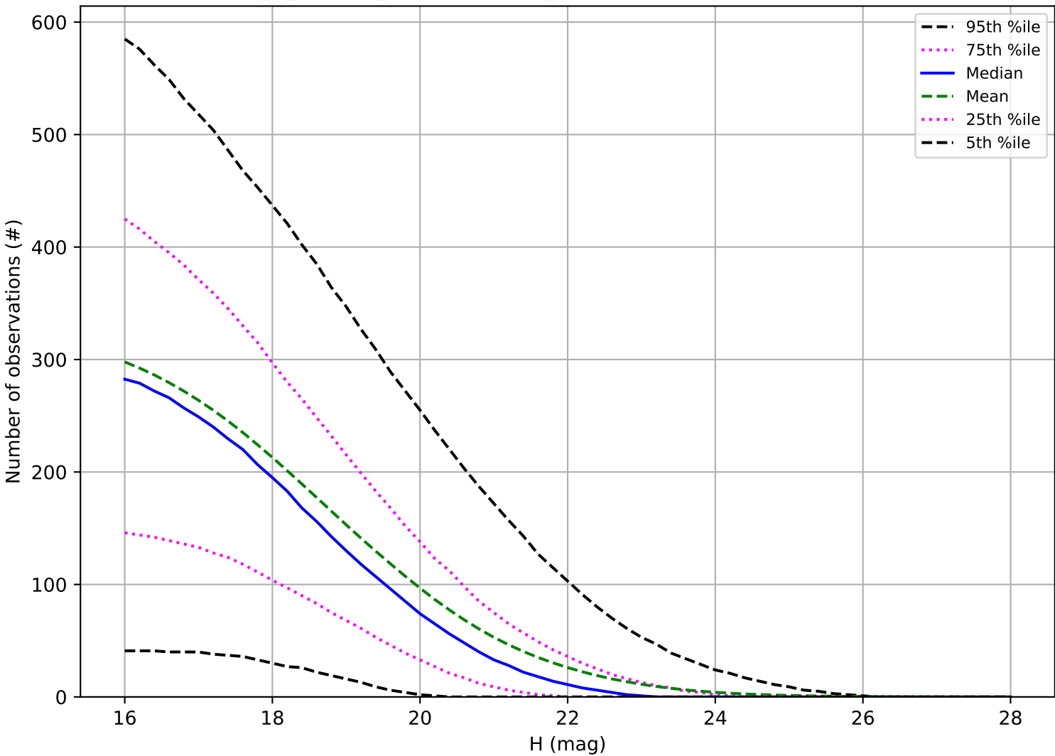
internal_u_expt30_nscale1.5v3.4_10yrs: Number of observations PHA
