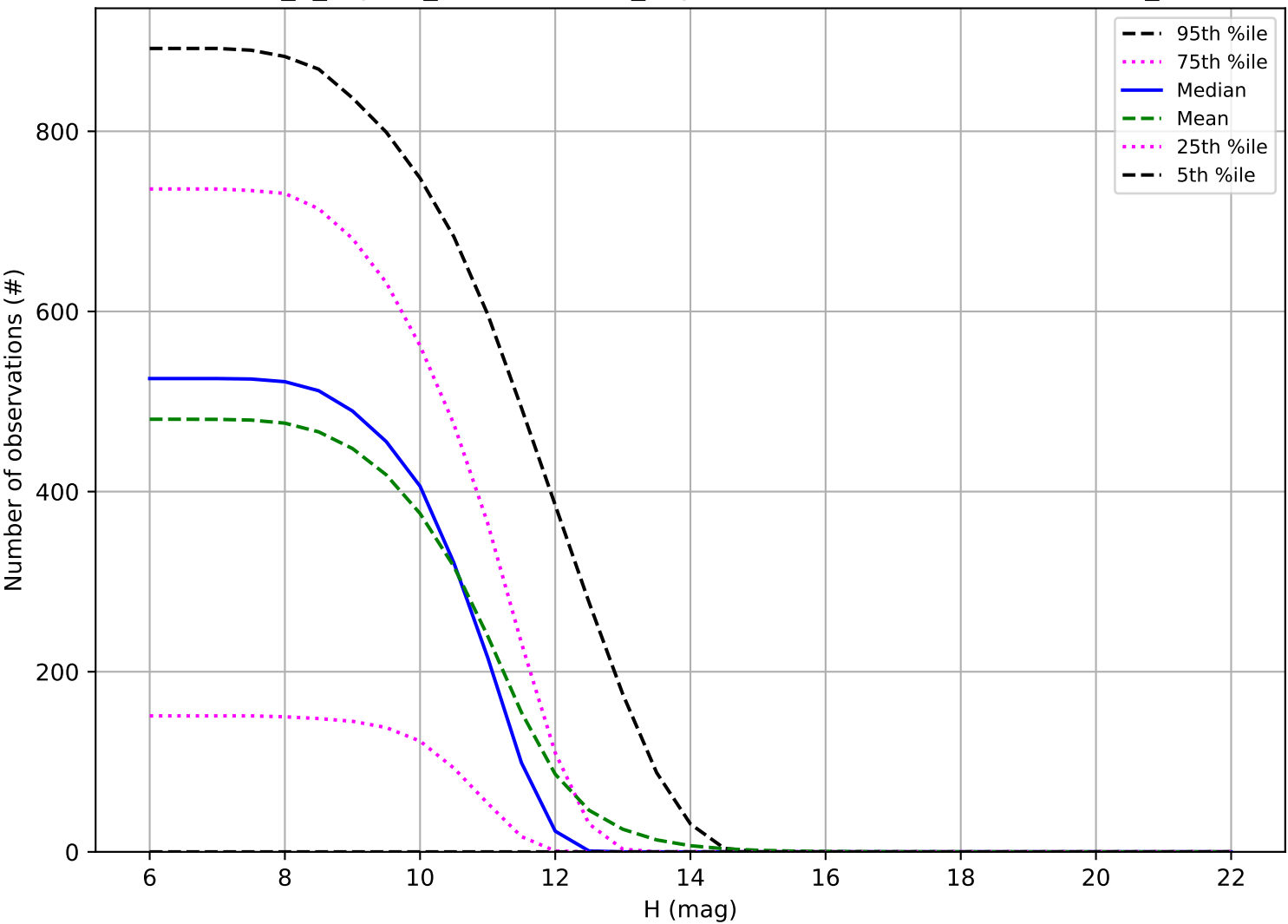
internal_u_expt30_nscale1.5v3.4_10yrs: Number of observations OCC_r20
