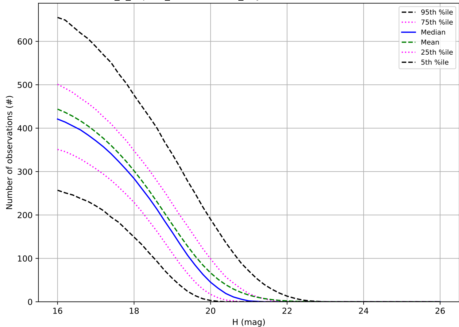
internal_u_expt30_nscale1.5v3.4_10yrs: Number of observations MBA
