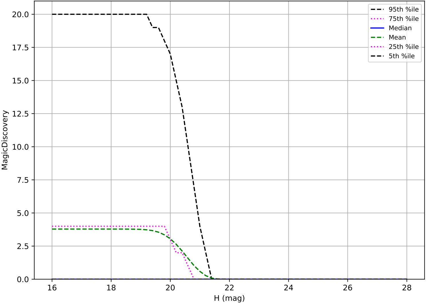
internal_u_expt30_nscale1.5v3.4_10yrs: Vatira 6 detections in 60 nights detection loss
