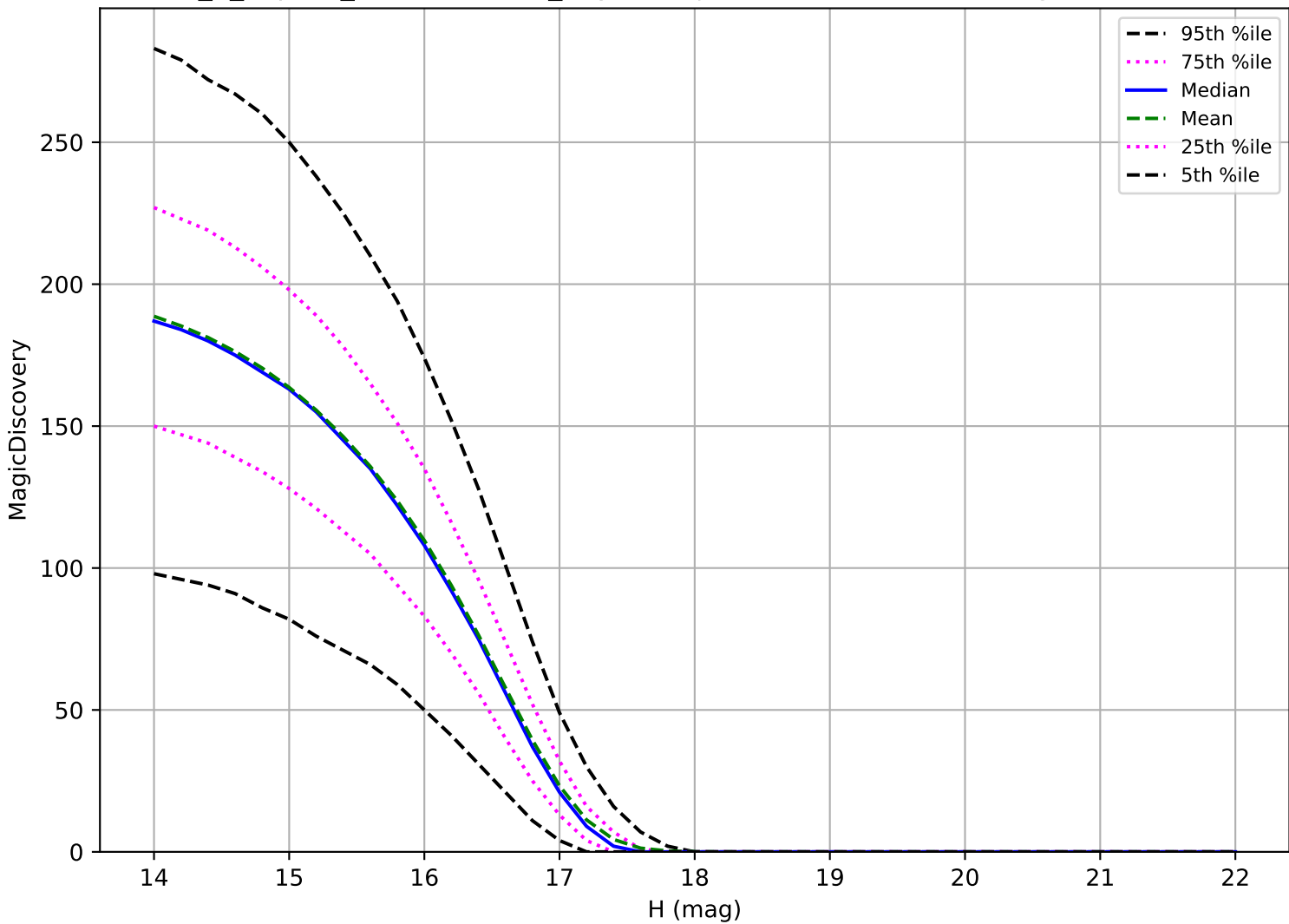
internal_u_expt30_nscale1.5v3.4_10yrs: Trojan 6 detections in 60 nights detection loss
