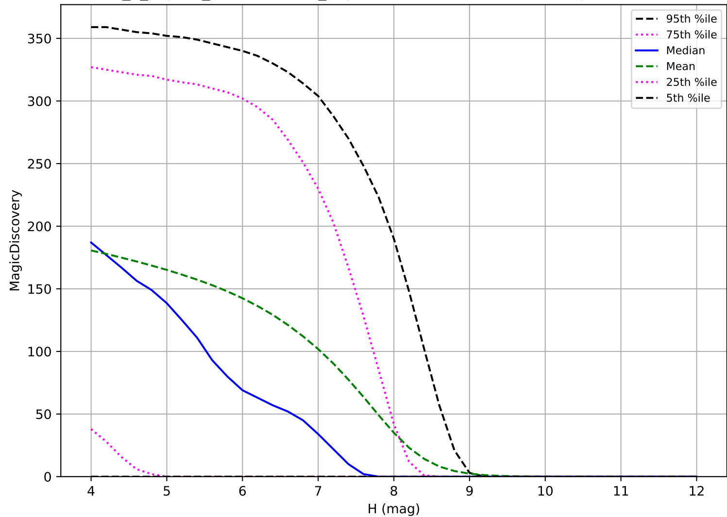
internal_u_expt30_nscale1.5v3.4_10yrs: TNO 6 detections in 60 nights detection loss
