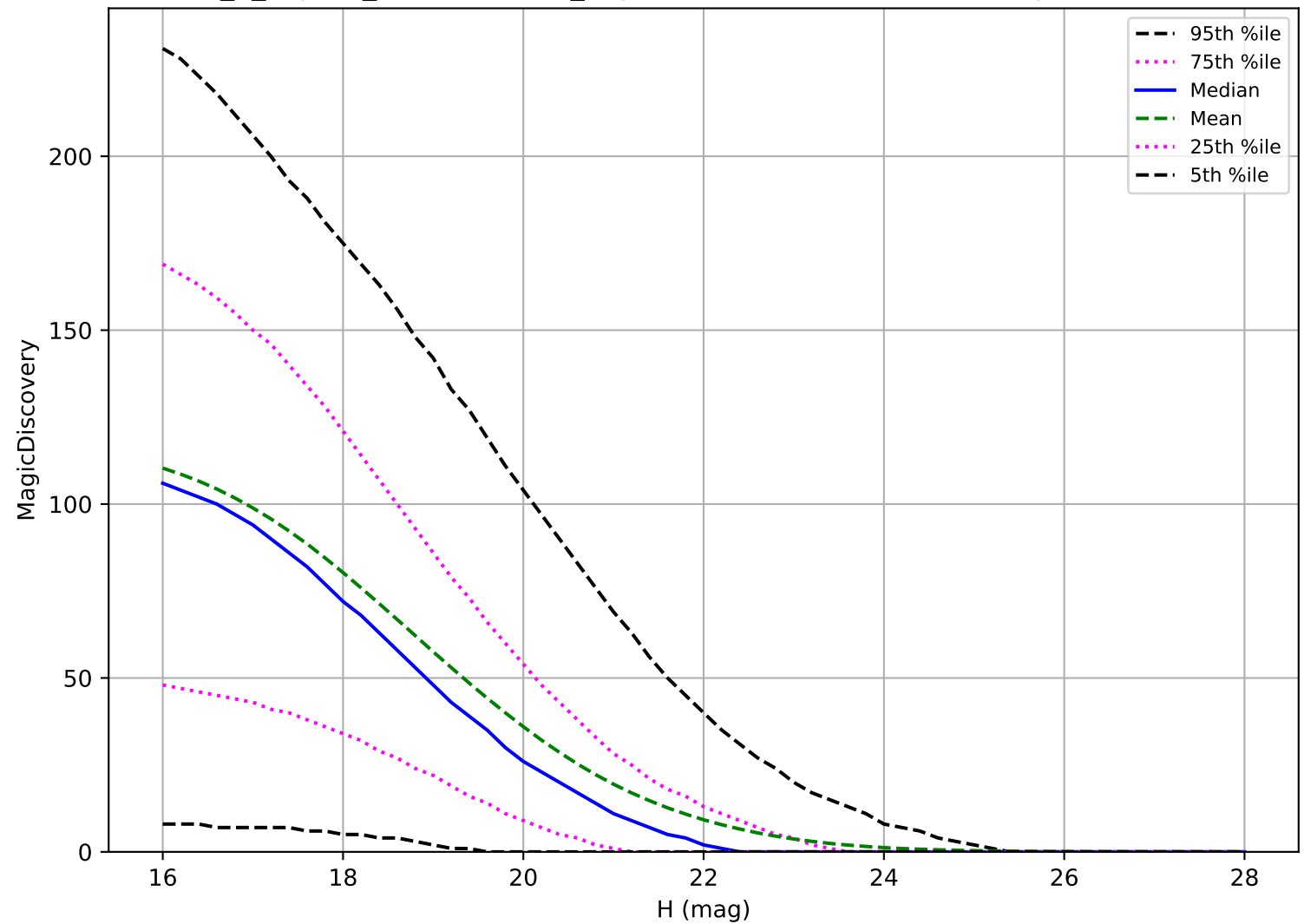
internal_u_expt30_nscale1.5v3.4_10yrs: PHA 6 detections in 60 nights detection loss
