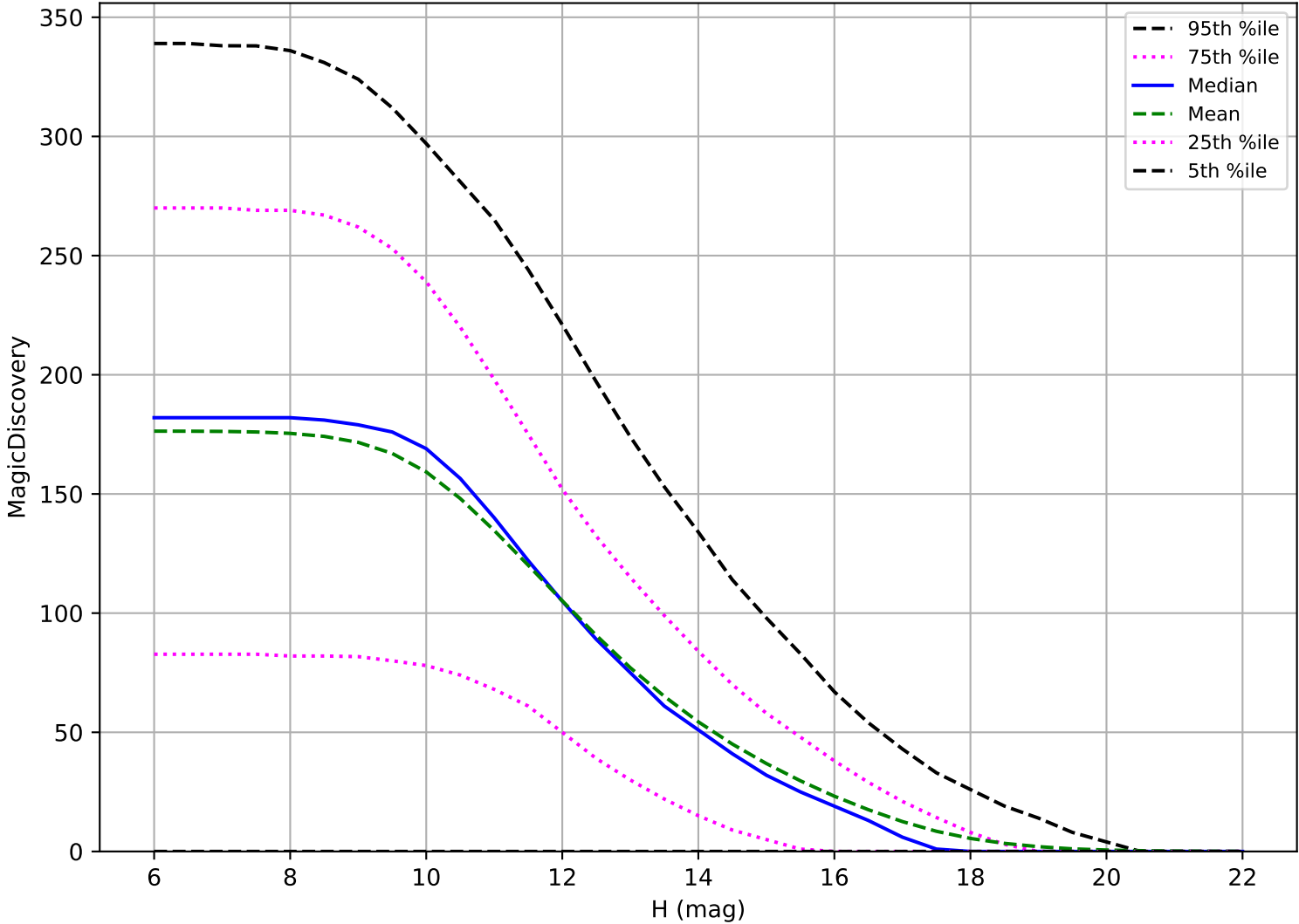
internal_u_expt30_nscale1.5v3.4_10yrs: OCC_r5 6 detections in 60 nights detection loss
