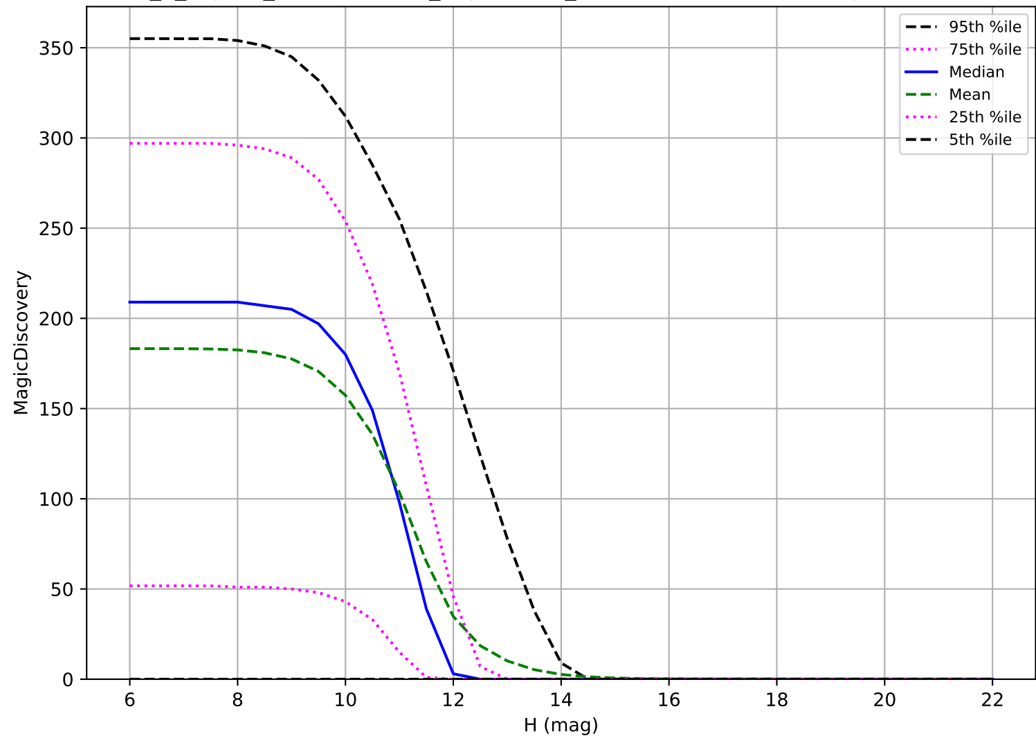
internal_u_expt30_nscale1.5v3.4_10yrs: OCC_r20 6 detections in 60 nights detection loss
