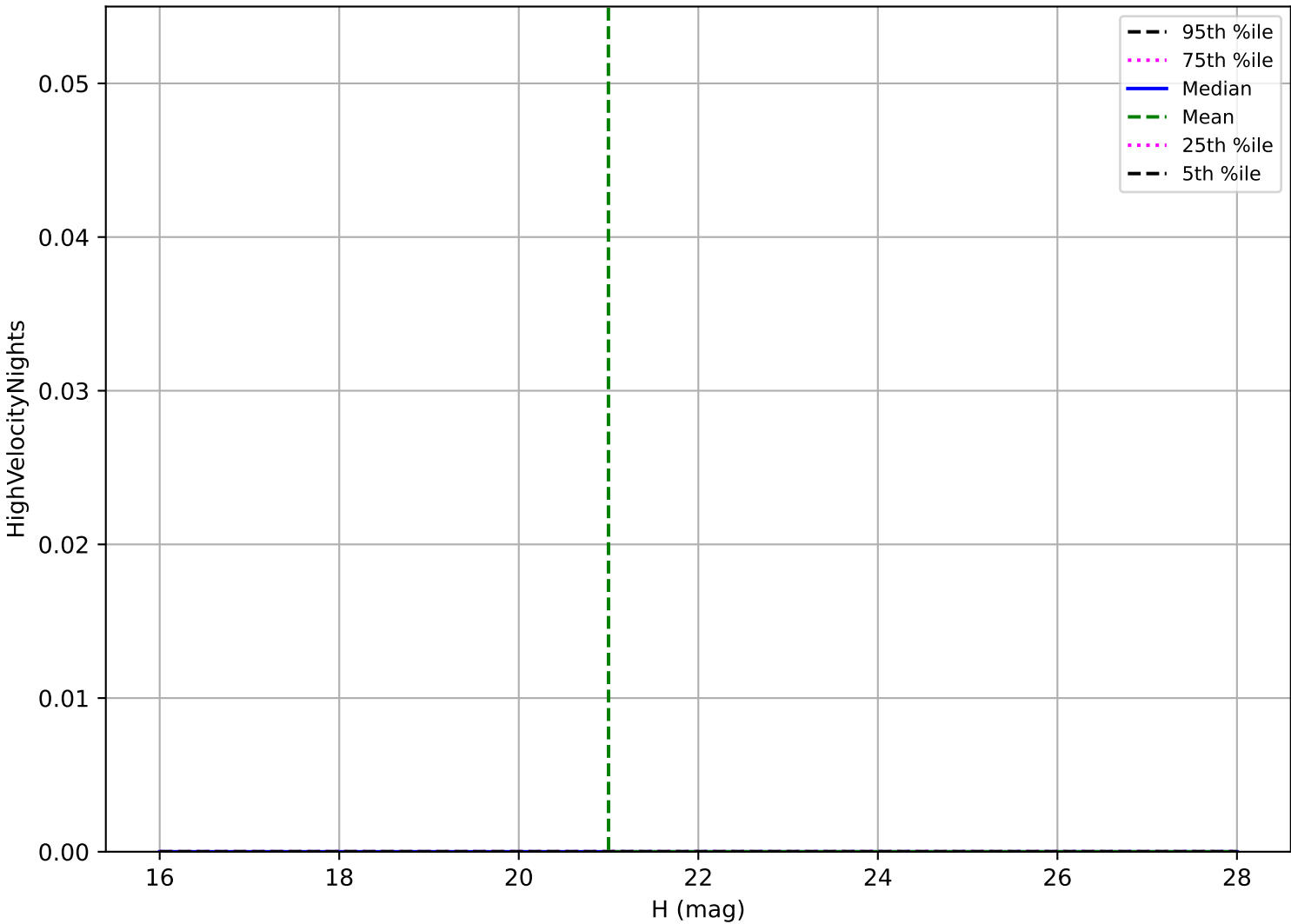
internal_u_expt30_nscale1.5v3.4_10yrs: Vatira High velocity pair detection loss
